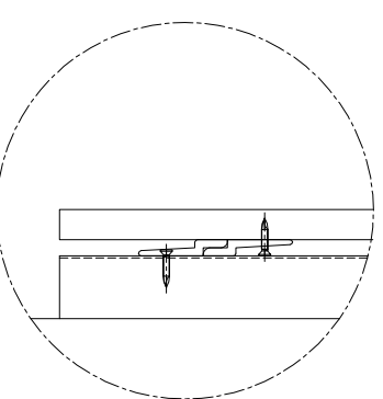
Detail B - 1:10
